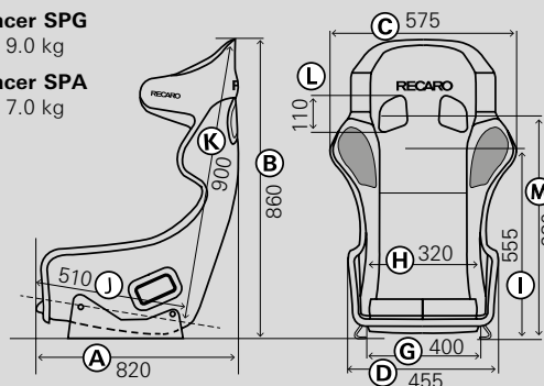
Picture with fixed steel sidemount
