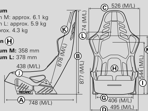
Picture with fixed steel sidemount
